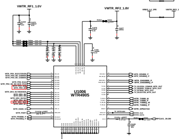
RF Transceiver
